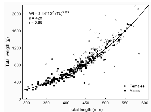
Figure 2. Length – weight relationship of female and male of gafttopsail catfish, Bagre marinus .
